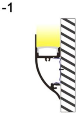
Installation steps
