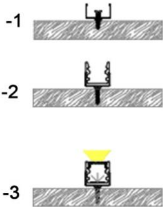
Installation steps
