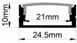
Dimension
