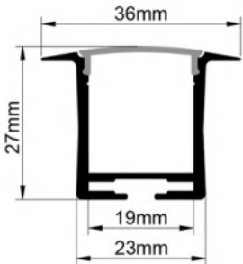
Dimension
