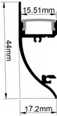
Dimension
