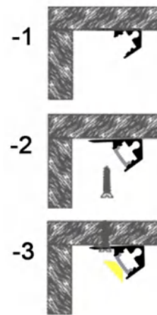
Installation steps
