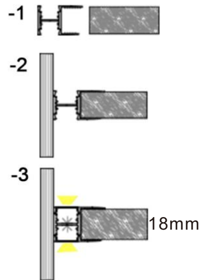
Installation steps
