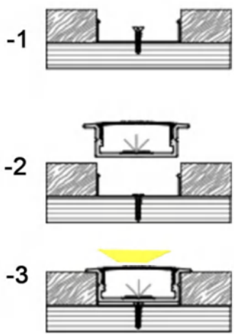
Installation steps
