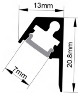
Dimension
