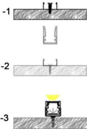
Installation steps
