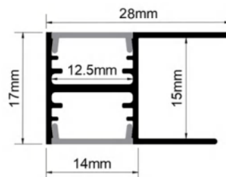
Dimension
