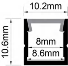
Dimension
