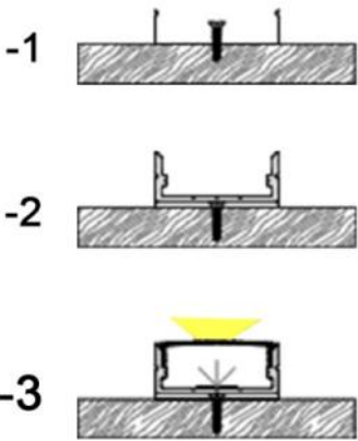
Installation steps
