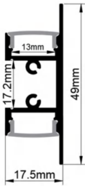
Dimension
