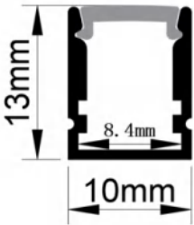
Dimension
