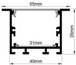
Dimension
