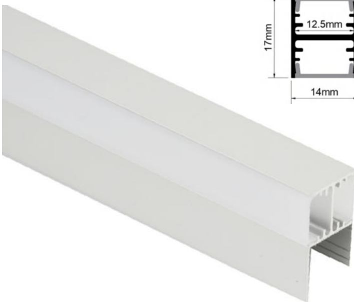
Dimension
